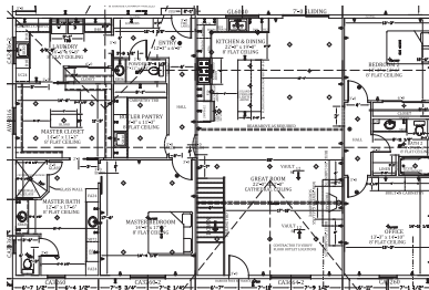
RESIDENCE / PLAN EXCERPT
